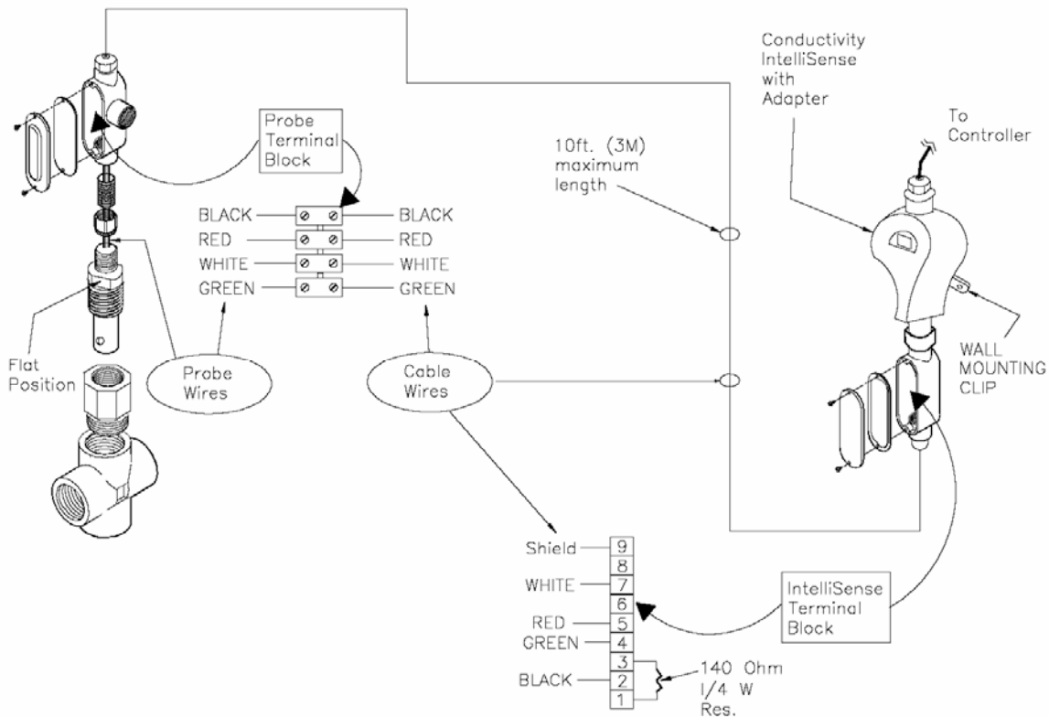
Fig. 6 Boiler probe
