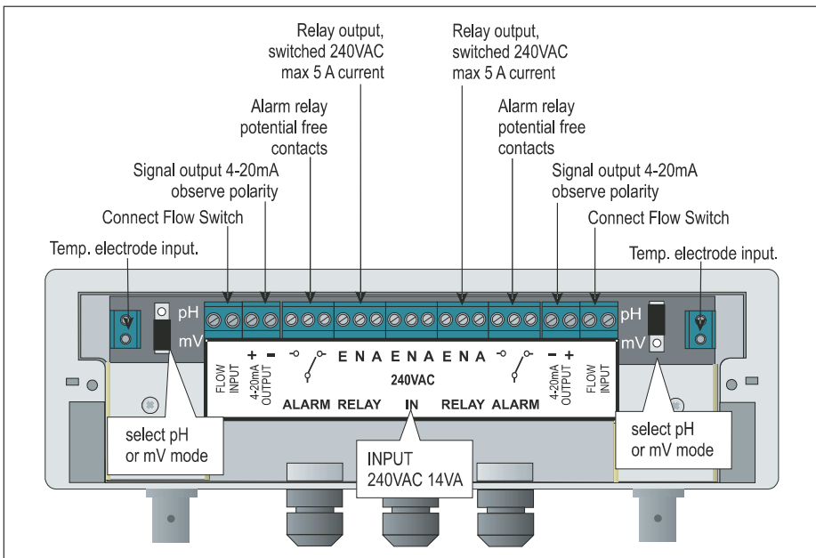
FIG 4 Terminal layout for the DPH-4
